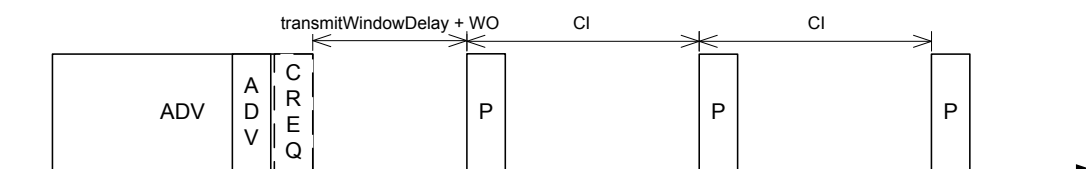
Figure 46: Peripheral connection setup and connection
