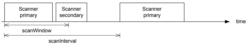
Figure 40: Scanner timing - a secondary scan timing-event does not have to fit within the scanWindow
