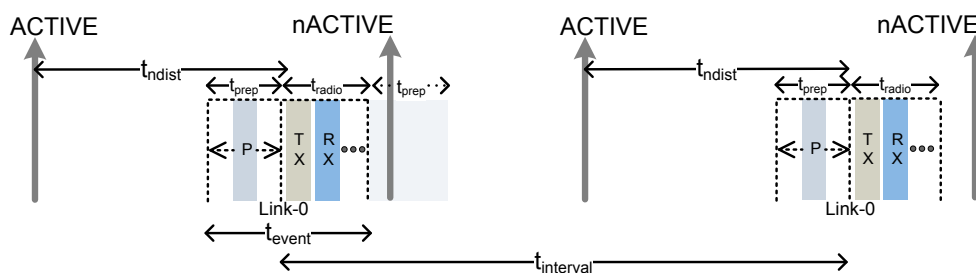
Figure 11: Radio Notification signal in relation to a single active link
