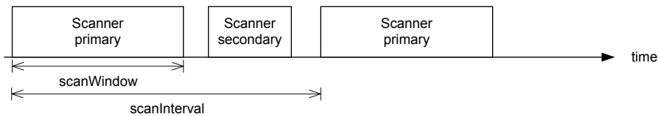
Figure 41: Scanner timing - a secondary scan timing-event may occur between two primary channel timing-events
