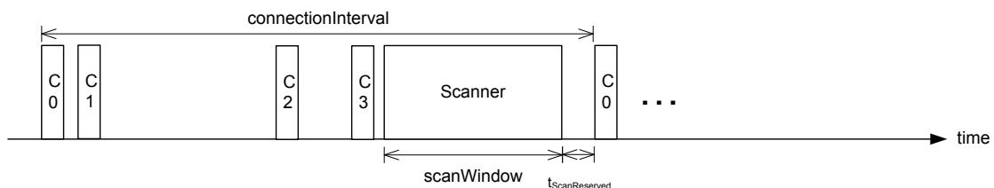
Figure 37: Scanner timing - always after connections
