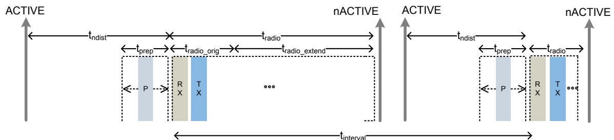
Figure 14: Peripheral connection event length extension limited by Radio Notification
