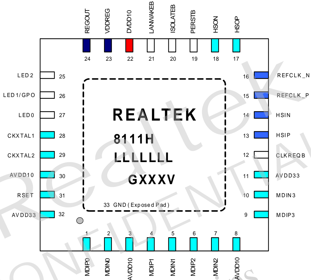
Figure 2. RTL8111H Pin Assignments
