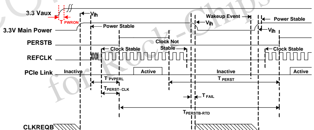
Figure 13. Auxiliary Signal Timing
